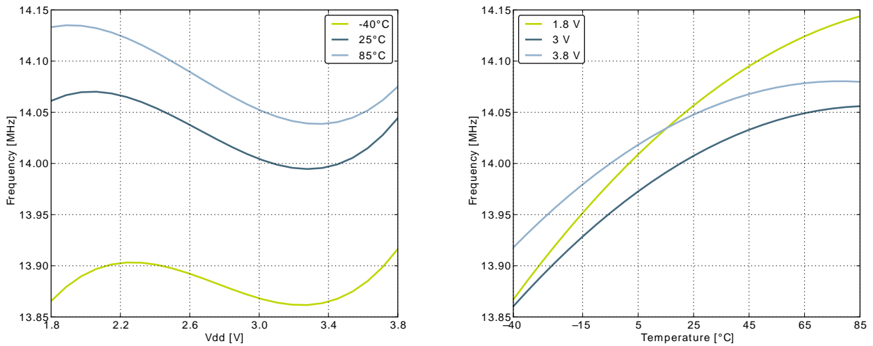
Figure 3.11. Calibrated HFRCO 21 MHz Band Frequency vs Temperature and Supply Voltage
