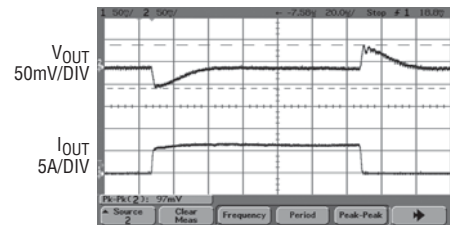
1.8V Transient Response
