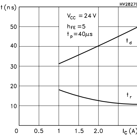
Figure 6. Switching times resistive on load
