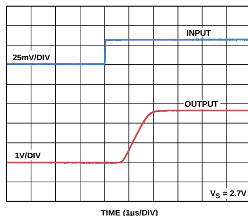
Figure 14. Differential Overload Recovery, Rising ( V_S = 2.7V )
