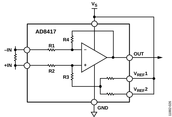
Figure 28. V_S Referenced Output
