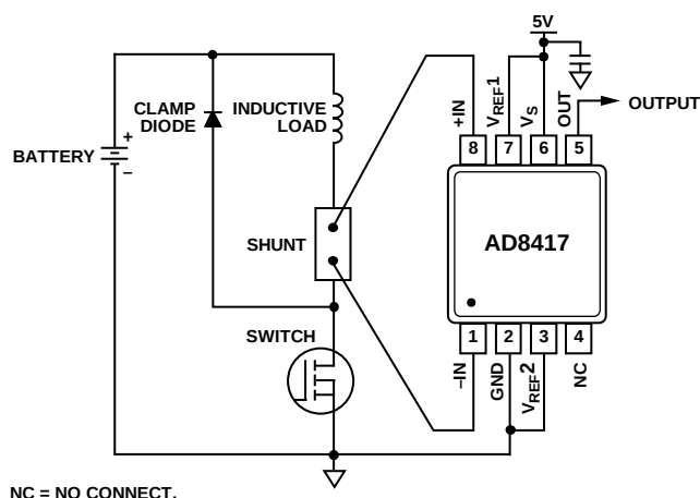
Figure 34. Low-Side Switch
