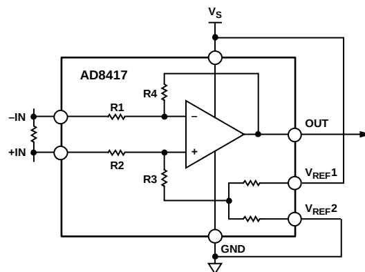
Figure 30. Split Supply
