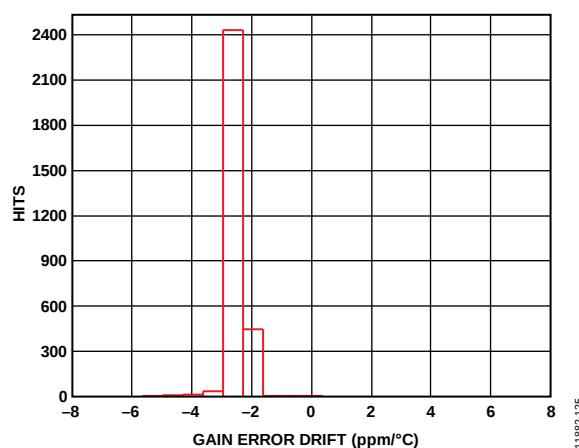
Figure 25. Gain Error Drift Distribution
