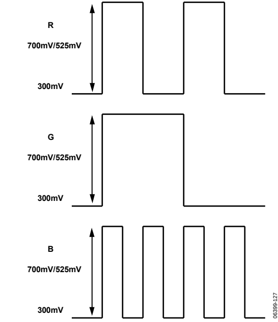
Figure 128. HD RGB Output Levels—RGB Sync Disabled
