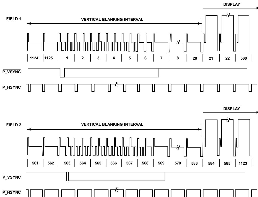
Figure 115. 1080i \overline{HSYNC} and \overline{VSYNC} Input Timing
