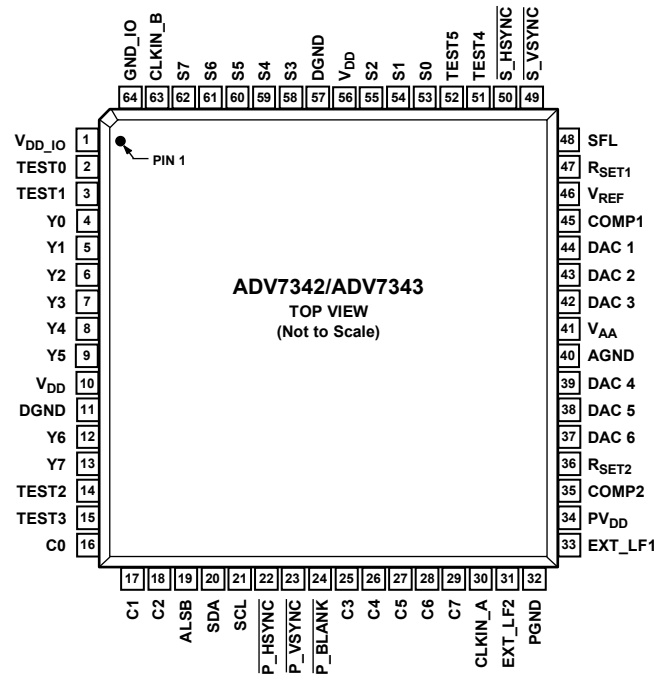
Figure 20. Pin Configuration
