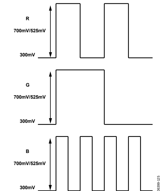
Figure 126. SD/ED RGB Output Levels—RGB Sync Disabled
