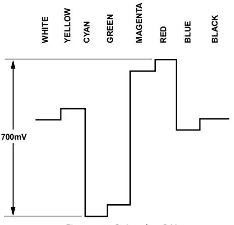
Figure 120. Pr Levels—PAL
