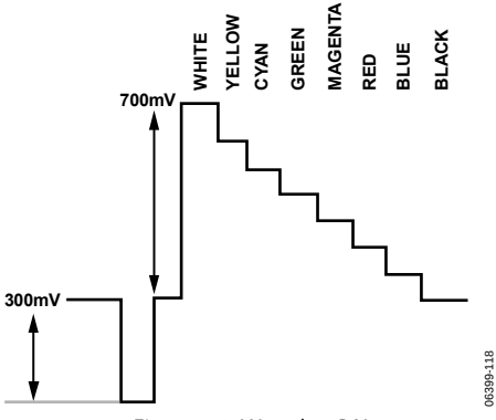
Figure 119. Y Levels—PAL
