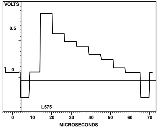
Figure 133. PAL Color Bars (75%)
