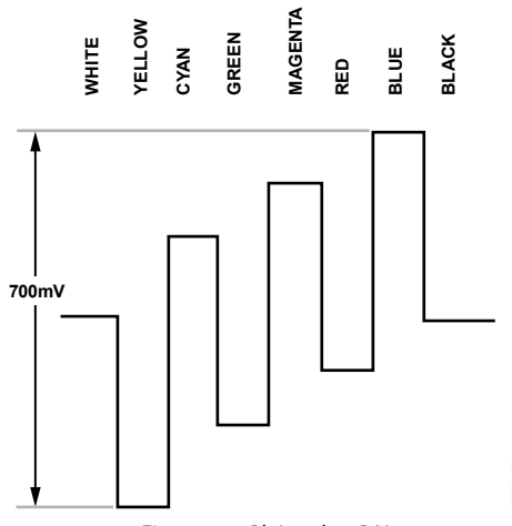
Figure 121. Pb Levels—PAL
