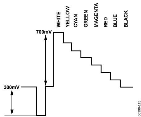
Figure 116. Y Levels—NTSC
