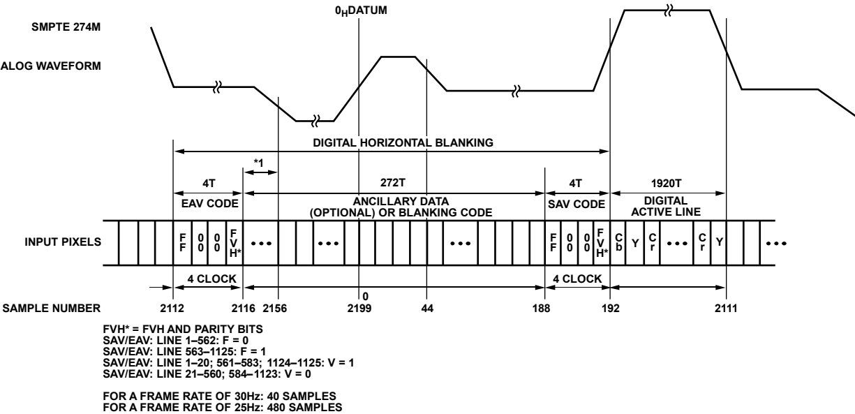
Figure 136. EAV/SAV Input Data Timing Diagram (SMPTE 274M)
