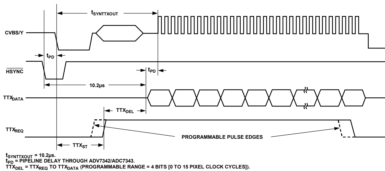
Figure 85. Teletext Functionality Diagram
