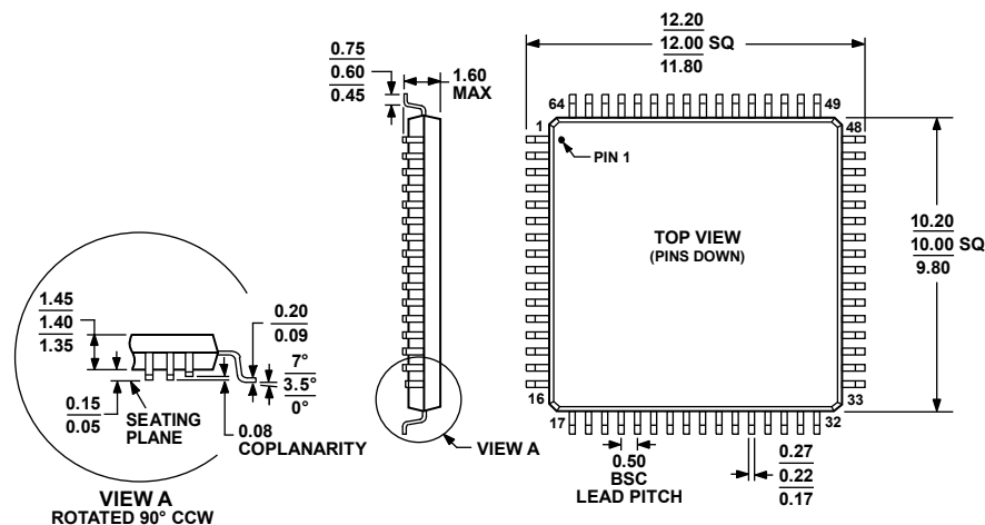
COMPLIANT TO JEDEC STANDARDS MS-026-BCD Figure 142. 64-Lead Low Profile Quad Flat Package [LQFP] (ST-64-2) Dimensions shown in millimeters
