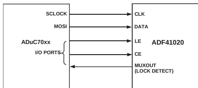
Figure 18. ADuC70xx-to-ADF41020 Interface
