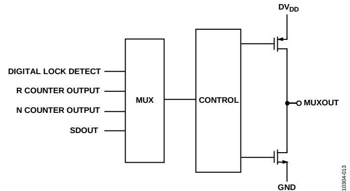
Figure 12. MUXOUT Circuit
