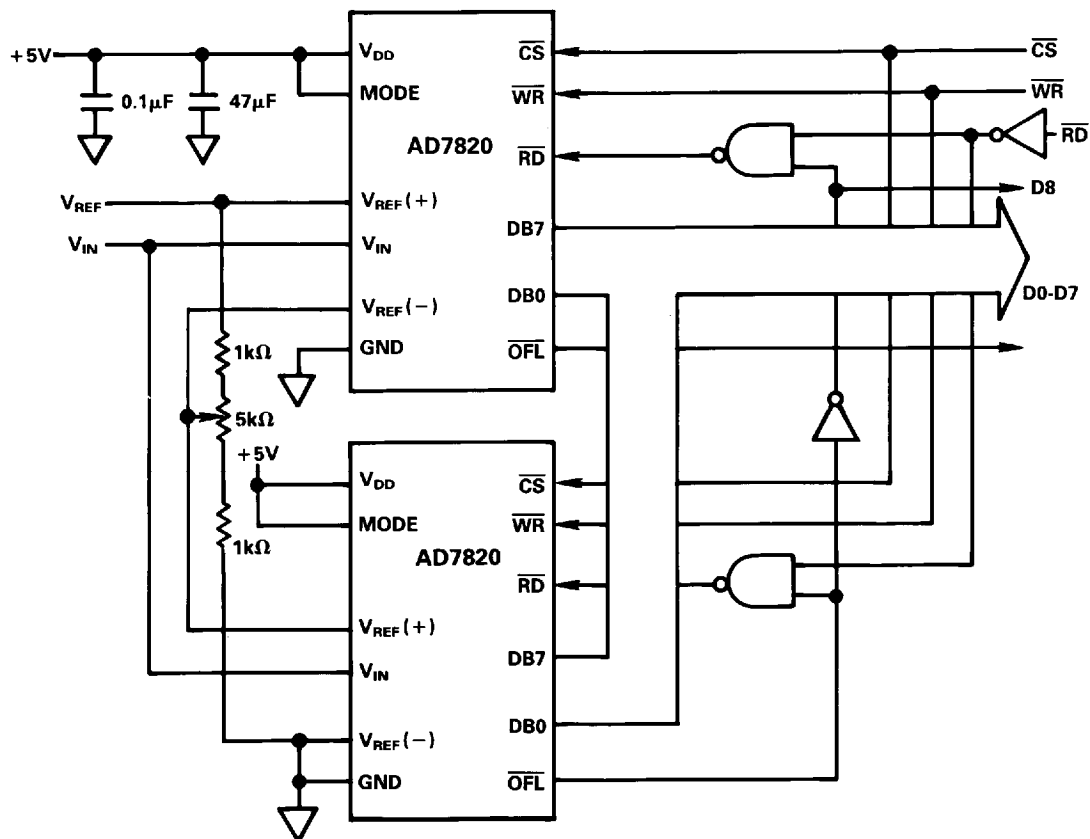
Figure 10. 9-Bit Resolution
