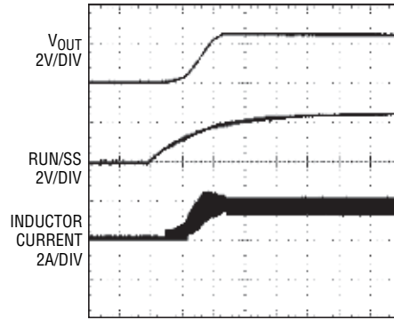
Start-Up Transient
