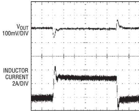
Load Step Transient Forced Continuous
