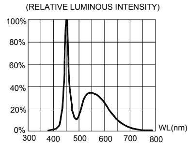
FIG.4 RELATIVE LUMINOUS INTENSITY VS. WAVELENGTH. 50% Power Angle : 105°
