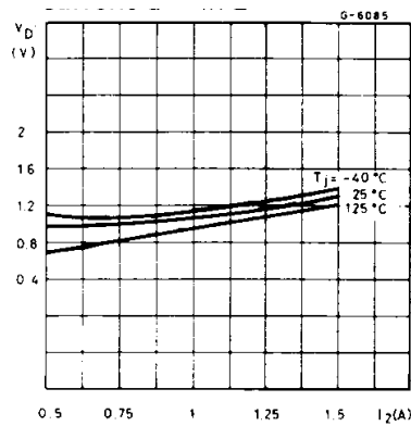
Figure 17. Dropout voltage between pin 1 and pin 2 vs. current at pin 2
