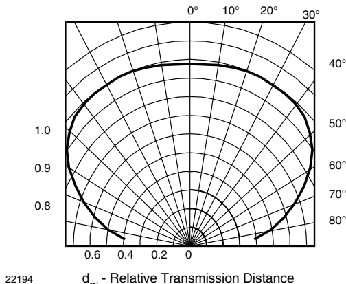
Fig. 12 - Vertical Directivity
