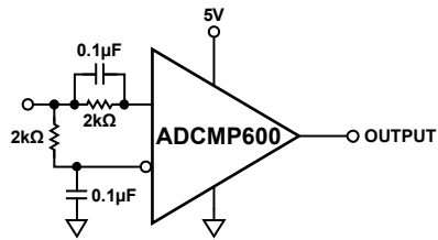
Figure 22. Self-Biased, 50% Slicer
