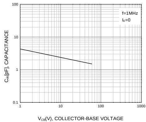
Figure 5. Output Capacitance
