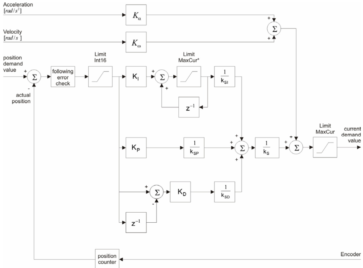
Figure 1: Controller architecture
