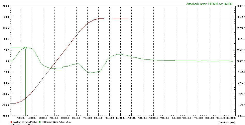
Figure 5: Recorded profile with stiff PID control
