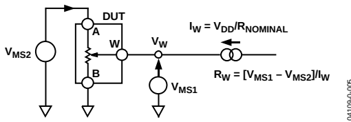
Figure 32. Test Circuit for Wiper Resistance
