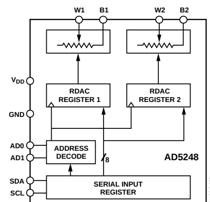
Figure 2. AD5248
