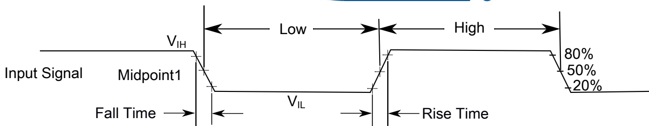
Figure 2. Input signal measurement reference
