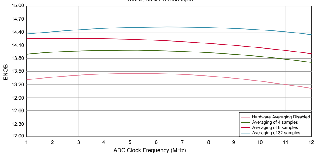
Figure 15. Typical ENOB vs. ADC_CLK for 16-bit differential mode
