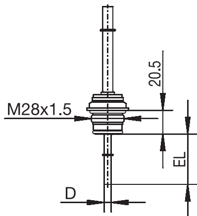
Varivent connection
