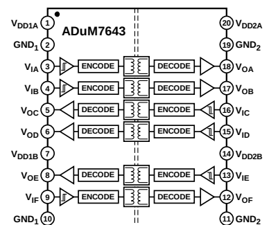
Figure 4. ADuM7643
