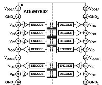
Figure 3. ADuM7642
