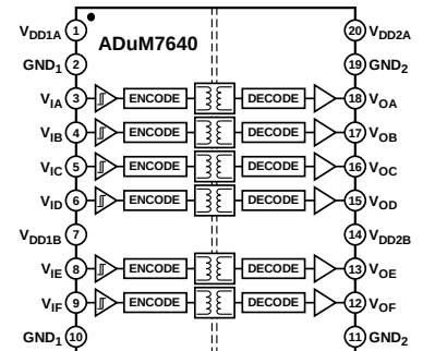
Figure 1. ADuM7640
