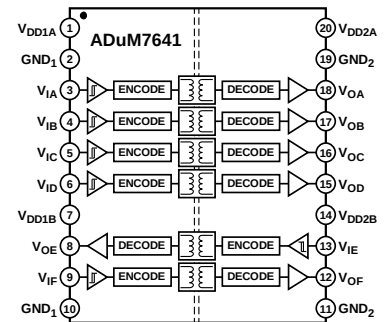
Figure 2. ADuM7641
