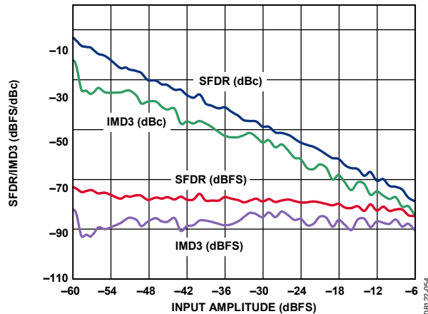
Figure 11. AD9204-80 Two-Tone SFDR/IMD3 vs. Input Amplitude (AIN) with f_{IN1} = 30.5 MHz and f_{IN2} = 32.5 MHz
