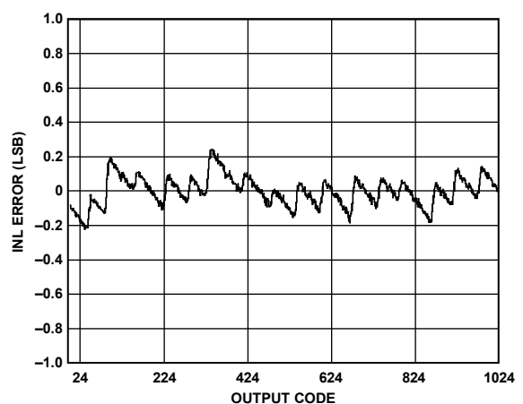
Figure 17. AD9204-80 INL with f_{IN} = 9.7\text{ MHz}
