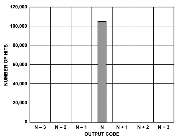
Figure 16. AD9204-80 Grounded Input Histogram
