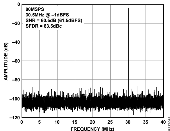
Figure 9. AD9204-80 Single-Tone FFT with f_{IN} = 30.5 MHz
