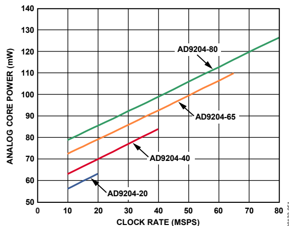
Figure 57. AD9204 Analog Core Power vs. Clock Rate
