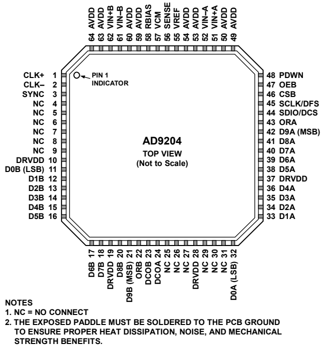
Figure 5. Pin Configuration
