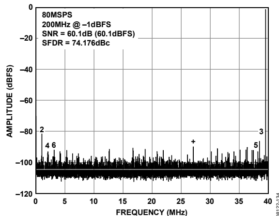
Figure 10. AD9204-80 Single-Tone FFT with f_{IN} = 200 MHz
