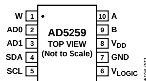
Figure 3. Pinout
