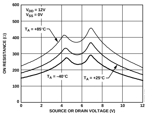
Figure 6. On Resistance as a Function of V_D ( V_S ) for Different Temperatures, Single Supply
