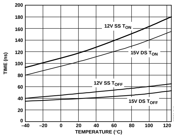
Figure 7. T_{ON}/T_{OFF} Times vs. Temperature
