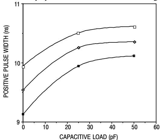
Figure 3. MC10H642 Positive PW versus Load @ \pm 5\% V_{CC} , T_A = 25^\circ\text{C}
