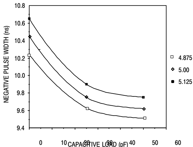
Figure 6. MC10H642 Negative PW versus Load @ \pm 2.5\% V_{CC} , T_A = 25^\circ\text{C}
