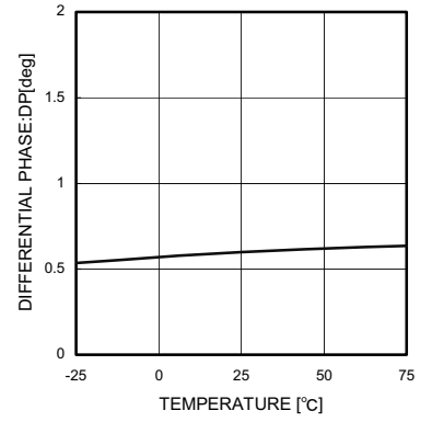
Fig.11 Differential Phase
