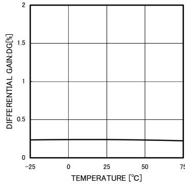
Fig.16 Differential Gain
