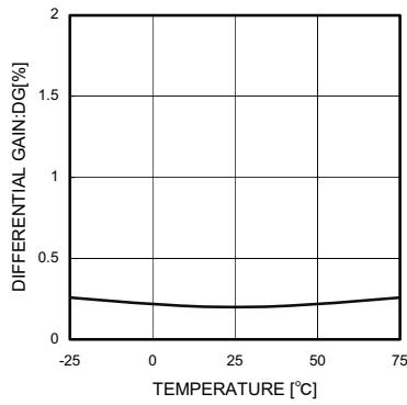
Fig.13 Differential Gain
