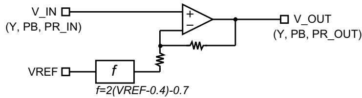
Fig. 4 DC_Shift block equivalent circuit
