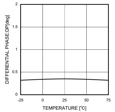
Fig.14 Differential Phase
