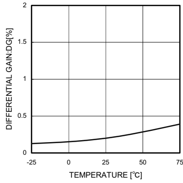
Fig.10 Differential Gain
