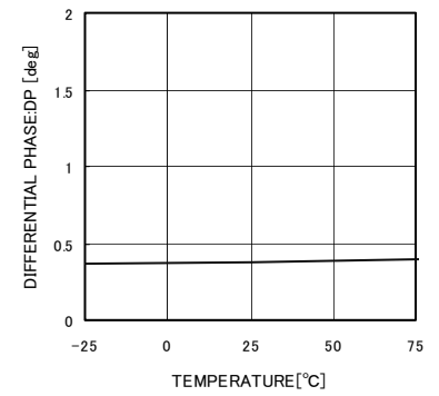
Fig.17 Differential Phase
