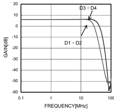
Fig.19 YLPF Characteristics
