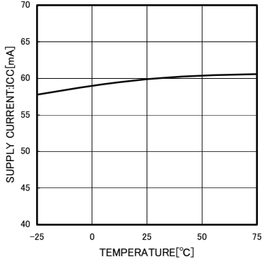
Fig.15 Circuit Current
