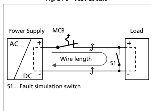
Fig. 24-5 Test circuit
