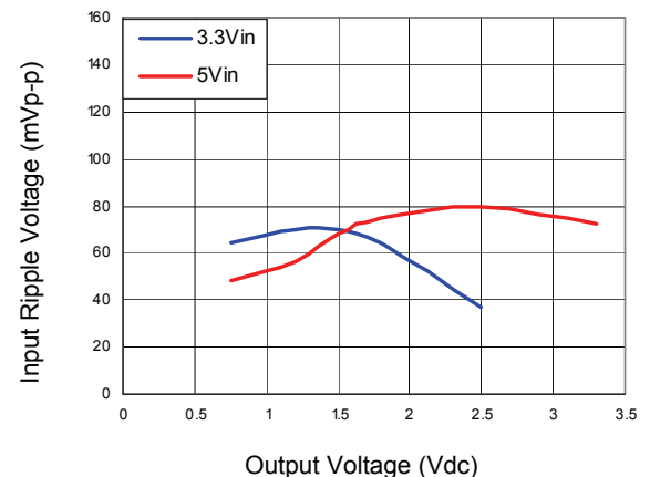
Figure 29. Input ripple voltage for various outputs with 1 \times 47\mu F ceramic capacitor at the input (full load).
