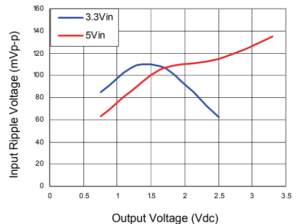
Figure 28. Input ripple voltage for various outputs with 1 \times 22\mu F ceramic capacitor at the input (full-load).
