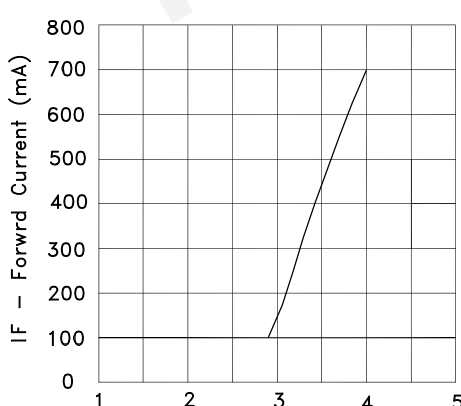
Forward Current Characteristics, Ta=25°C
