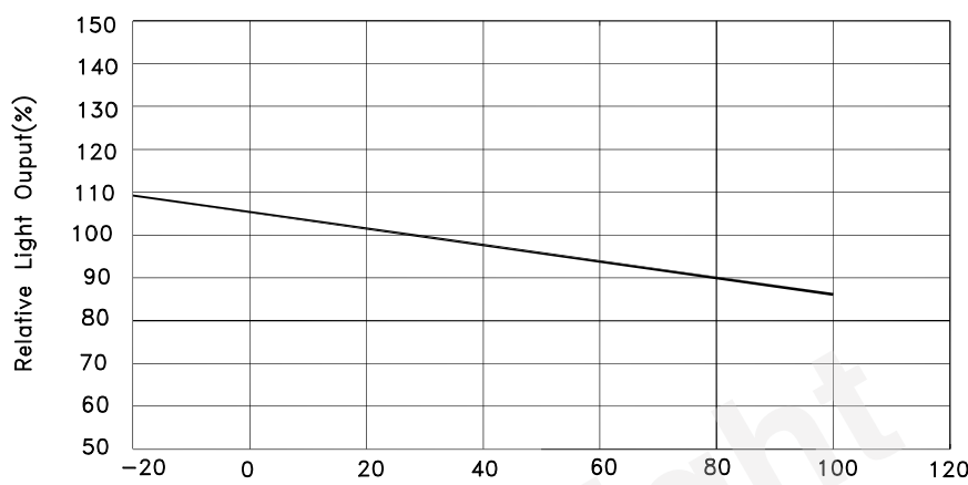
Light Output Characteristics
