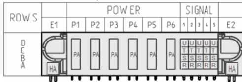
Female Connector: FCI (51732-020 LF)
