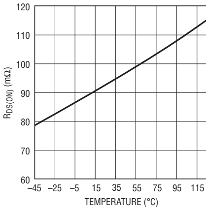
Switch R_{DS(ON)} vs Temperature
