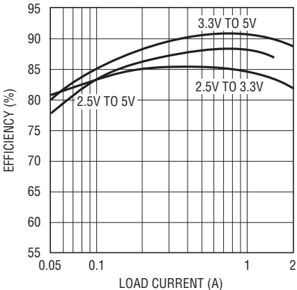
Converter Efficiency
