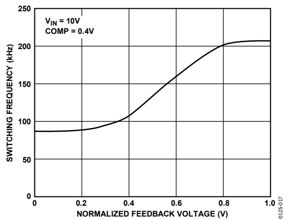
Figure 17. Frequency Foldback
