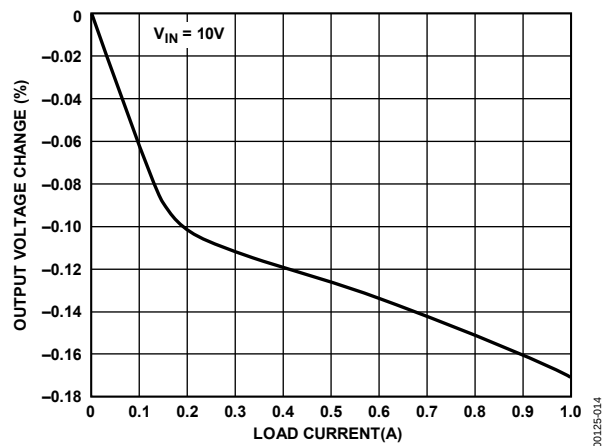
Figure 14. Load Regulation
