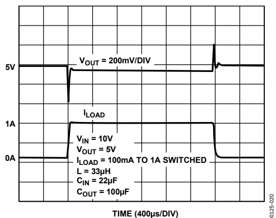
Figure 20. Transient Response
