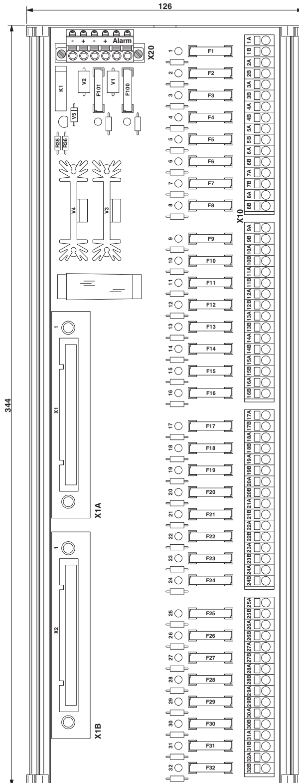
Dimensioned drawing
