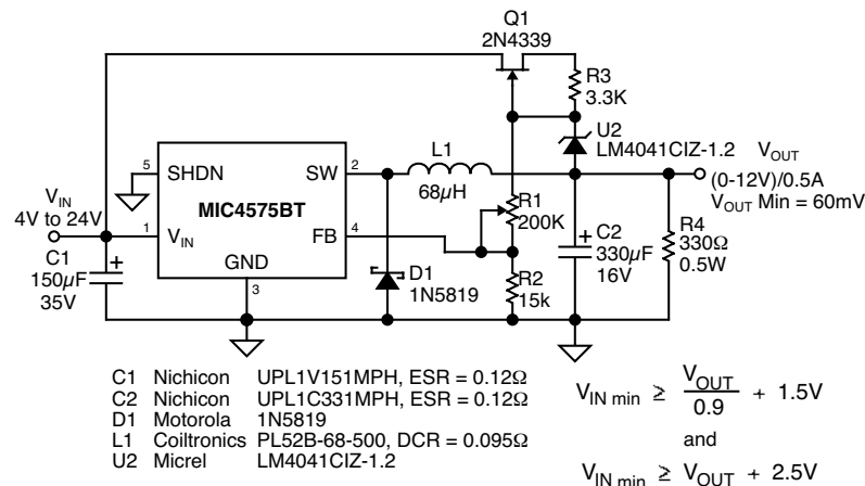
Figure 14. Adjustable (0V–12V) Output-Voltage Regulator
