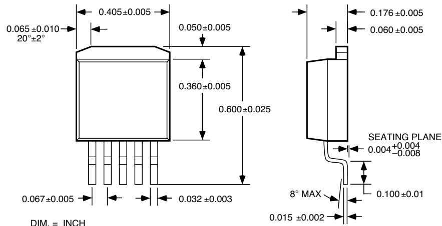
5-Lead TO-263 (U)
