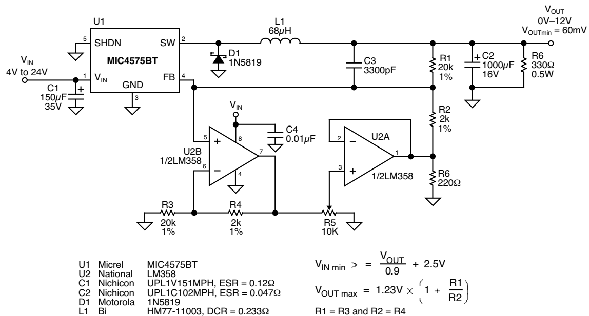
Figure 22. Improved Adjustable Output-Voltage Regulator (0V-12V)
