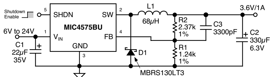
Adjustable Regulator
