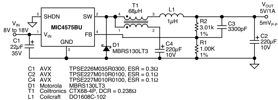
Figure 12. Low Output-Noise Regulator (5mV Output Ripple)
