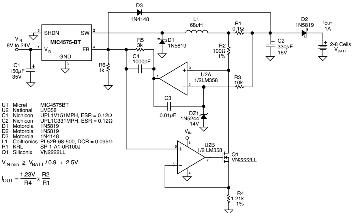
Figure 18. 1A Battery Charger (2-8 Cells)
