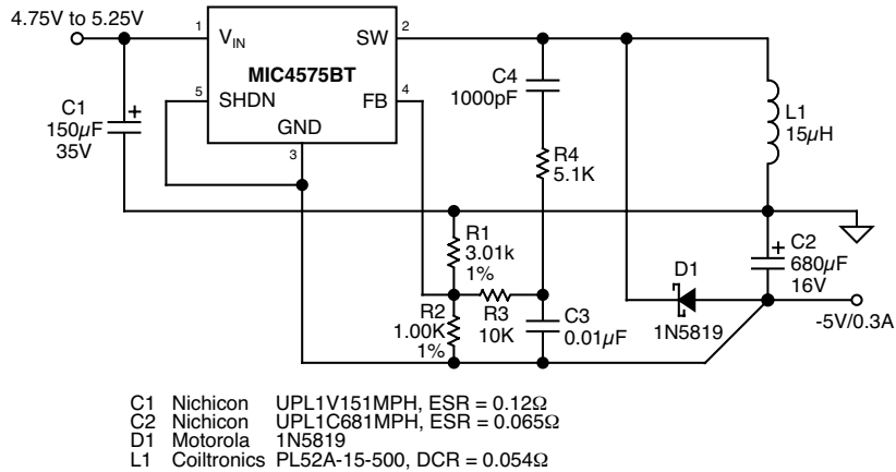
Figure 11. 5V to -5V/0.3A Buck-Boost Converter Through Hole
