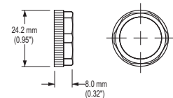
Figure 6. Lock Nut
