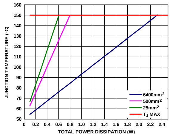
Figure 64. LFCSP, T_A = 50^\circ\text{C}
