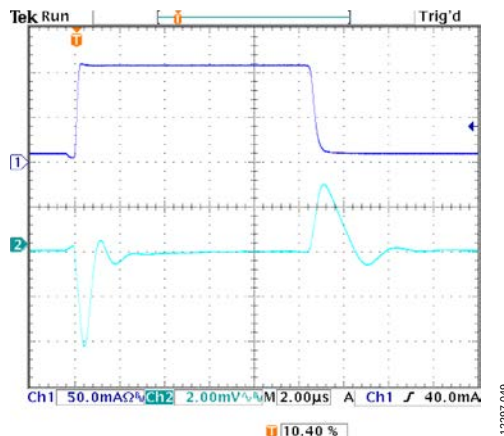
Figure 49. Load Transient Response, I_{LOAD} = 10\text{ mA} to 110\text{ mA} , V_{OUT} = 5\text{ V} , V_{IN} = 5.5\text{ V} , CH1 = I_{LOAD} , CH2 = V_{OUT}
