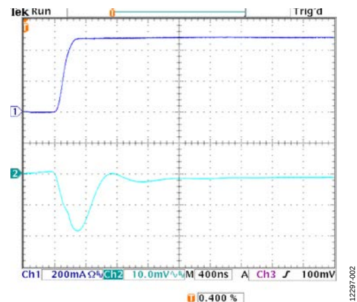
Figure 2. Transient Response (Trace 2), 1 mA to 500 mA Load Step in 400 ns (Trace 1)
