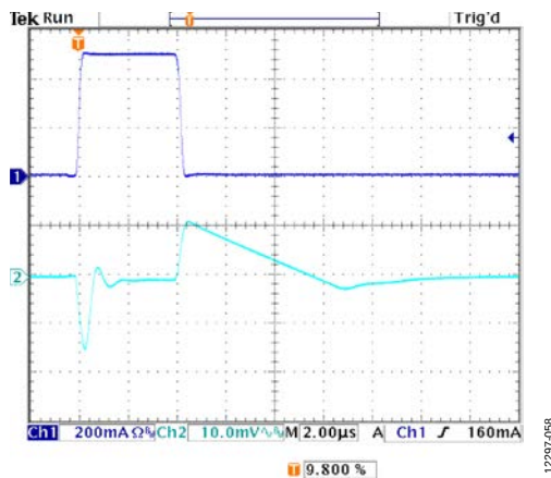
Figure 56. Output Transient Response, V_{\text{OUT}} = 5\text{ V} , C_{\text{OUT}} = 4.7\text{ }\mu\text{F}
