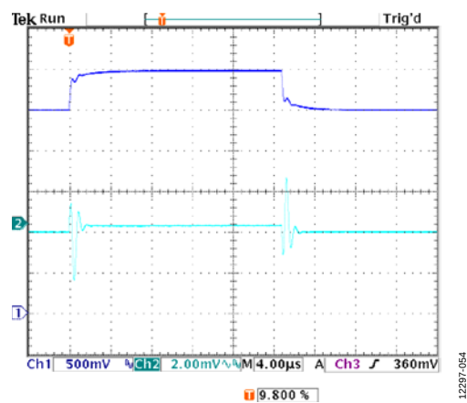
Figure 53. Line Transient Response, 2.5 V to 3 V, I_{LOAD} = 500 mA, Adjustable Version, V_{OUT} = 1.2 V, CH1 = V_{IN} , CH2 = V_{OUT}
