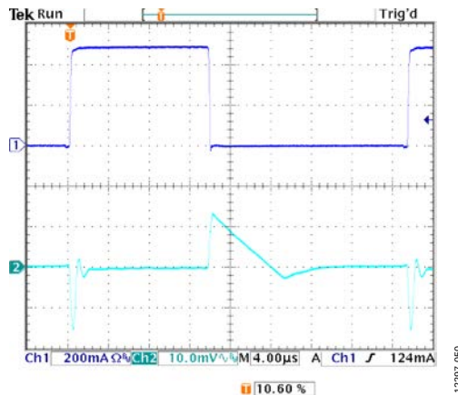
Figure 50. Load Transient Response, I_{LOAD} = 10\text{ mA} to 510\text{ mA} , Adjustable Version, V_{OUT} = 1.2\text{ V} , V_{IN} = 2.5\text{ V} , CH1 = I_{LOAD} , CH2 = V_{OUT}
