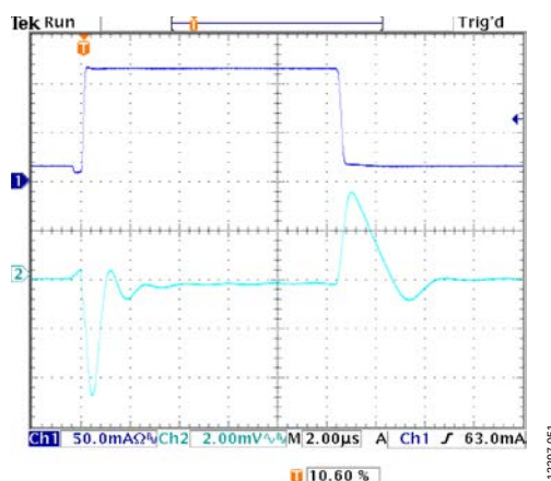
Figure 51. Load Transient Response, I_{LOAD} = 10\text{ mA} to 110\text{ mA} , Adjustable Version, V_{OUT} = 1.2\text{ V} , V_{IN} = 2.5\text{ V} , CH1 = I_{LOAD} , CH2 = V_{OUT}
