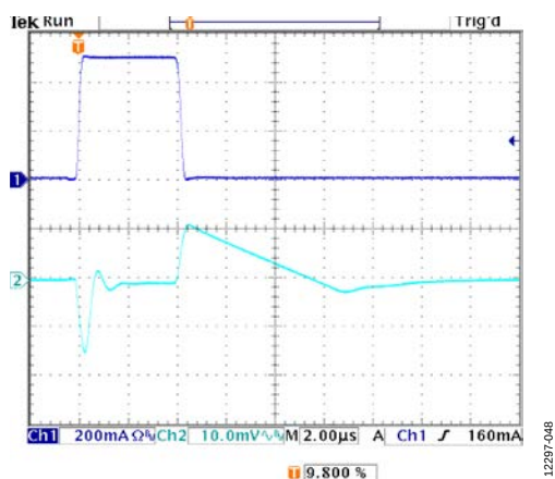
Figure 48. Load Transient Response, I_{LOAD} = 10\text{ mA} to 510\text{ mA} , V_{OUT} = 5\text{ V} , V_{IN} = 5.5\text{ V} , CH1 = I_{LOAD} , CH2 = V_{OUT}
