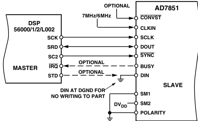
Figure 48. DSP56000/1/2/L002 Interface
