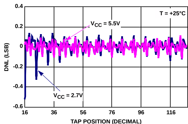
FIGURE 7. DNL vs TAP POSITION IN RHEOSTAT MODE FOR 10k \Omega (W)
