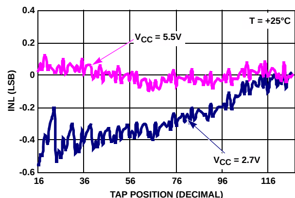
FIGURE 8. INL vs TAP POSITION IN RHEOSTAT MODE FOR 10k \Omega (W)
