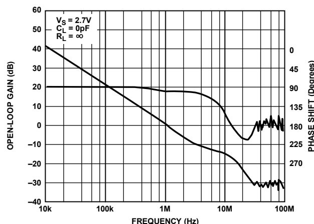
Figure 17. Open-Loop Gain and Phase Shift vs. Frequency
