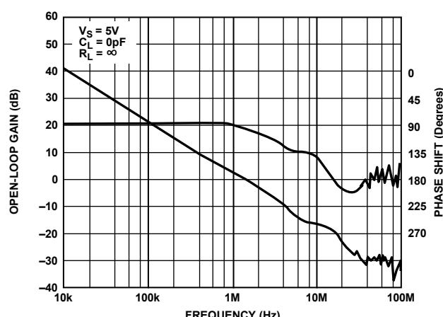
Figure 18. Open-Loop Gain and Phase Shift vs. Frequency
