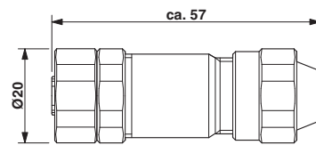
Dimensioned drawing
