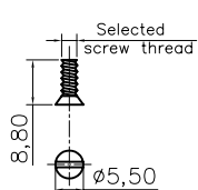
1 Screw x2
