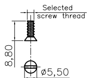
1 Screw x2
