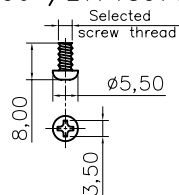
2 Screw x2
