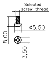
2 Screw x2
