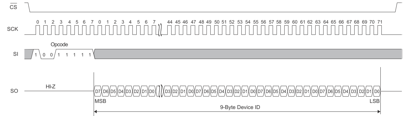
Figure 16. Read Device ID
