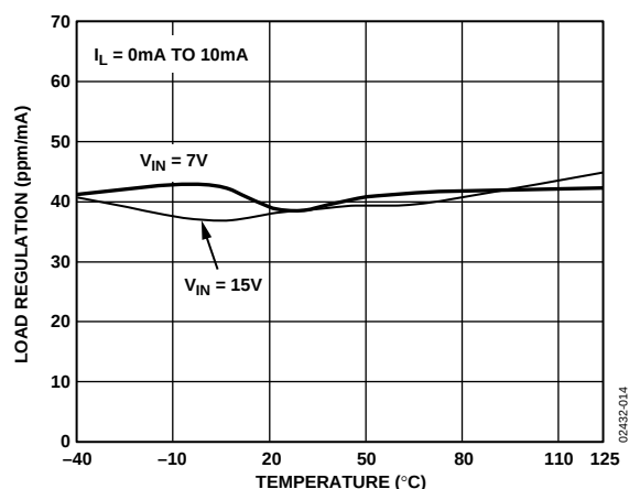
Figure 14. ADR423 Load Regulation vs. Temperature
