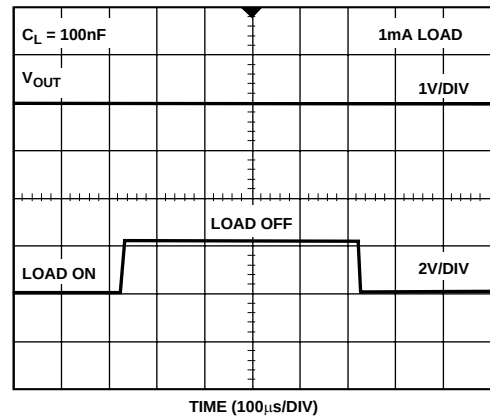
Figure 31. ADR421 Load Transient Response, C_L = 100\text{ nF}
