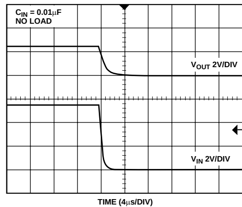
Figure 32. ADR421 Turn-Off Response
