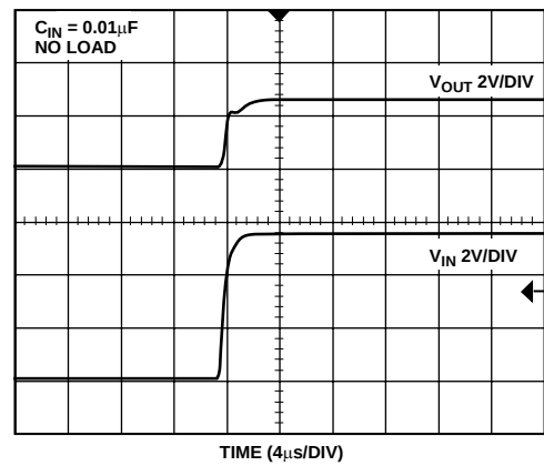
Figure 33. ADR421 Turn-On Response
