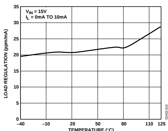
Figure 15. ADR425 Load Regulation vs. Temperature
