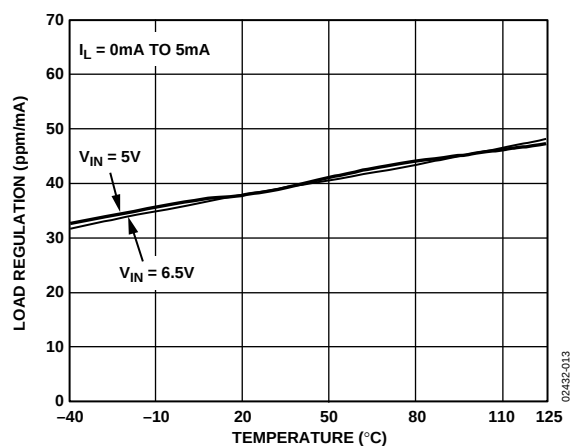
Figure 13. ADR421 Load Regulation vs. Temperature
