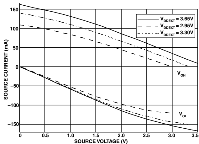
Figure 30. Drive Current B (High V_{DDEXT} )
