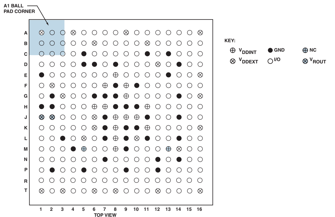
Figure 48. 256-Ball CSP_BGA Ball Configuration (Top View)
