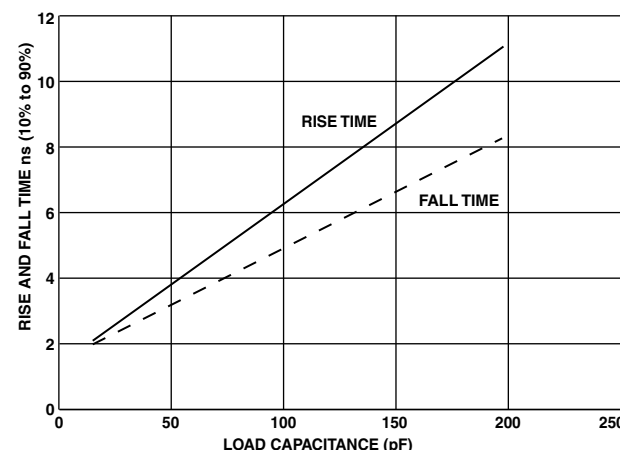
Figure 40. Typical Rise and Fall Times (10% to 90%) versus Load Capacitance for Driver B at V_{DDEXT} (min)
