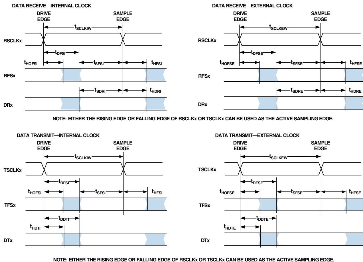
Figure 19. Serial Ports
