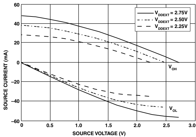
Figure 31. Drive Current C (Low V_{DDEXT} )
