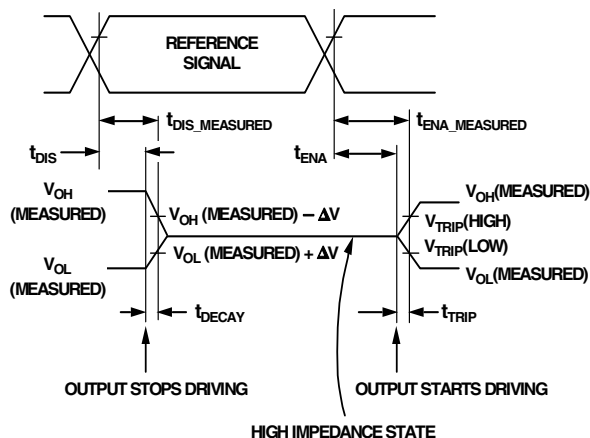
Figure 36. Output Enable/Disable
