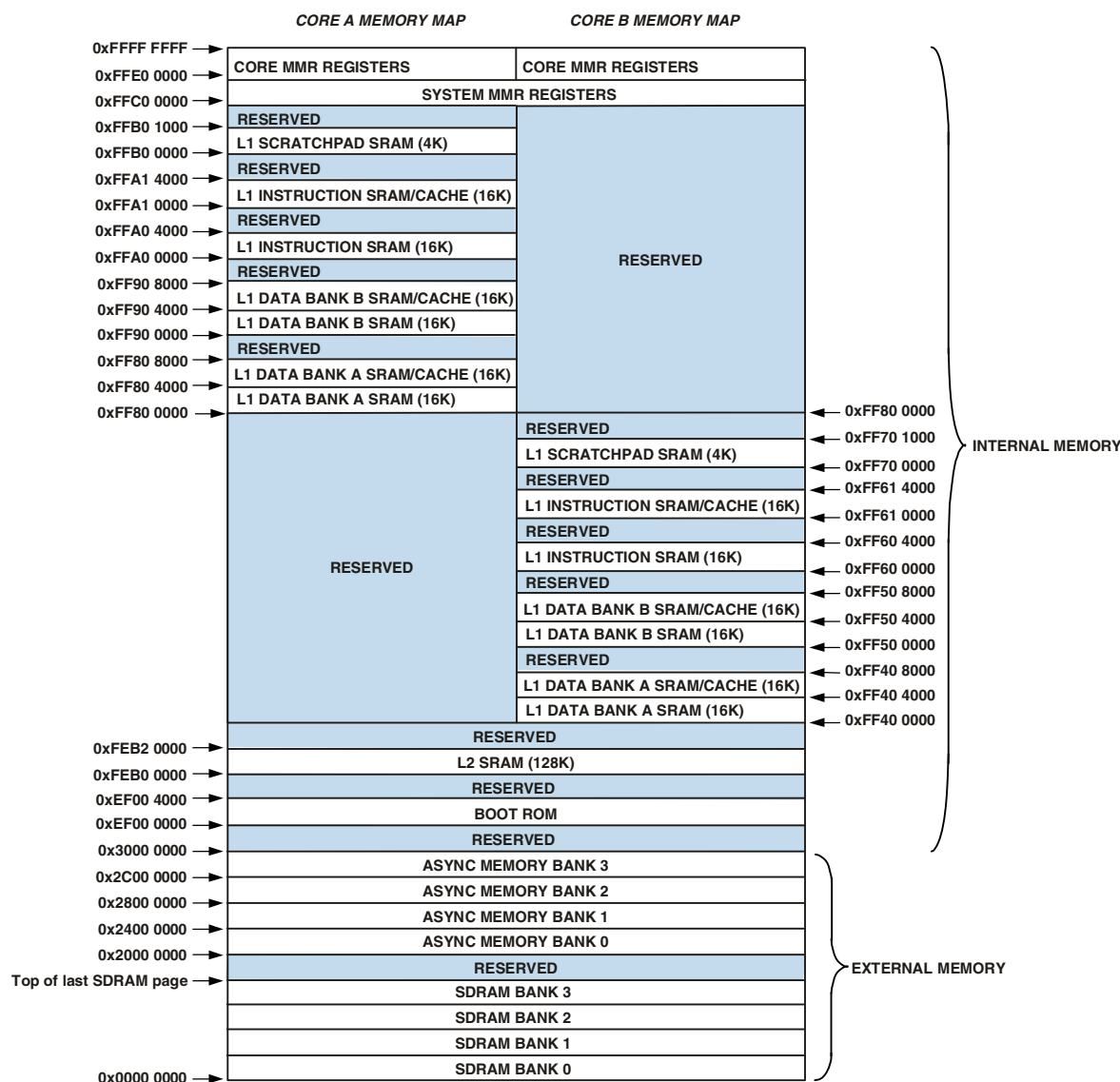
Figure 3. Memory Map
