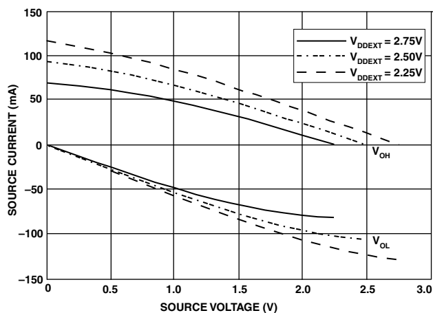
Figure 29. Drive Current B (Low V_{DDEXT} )
