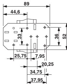
Dimensioned drawing
