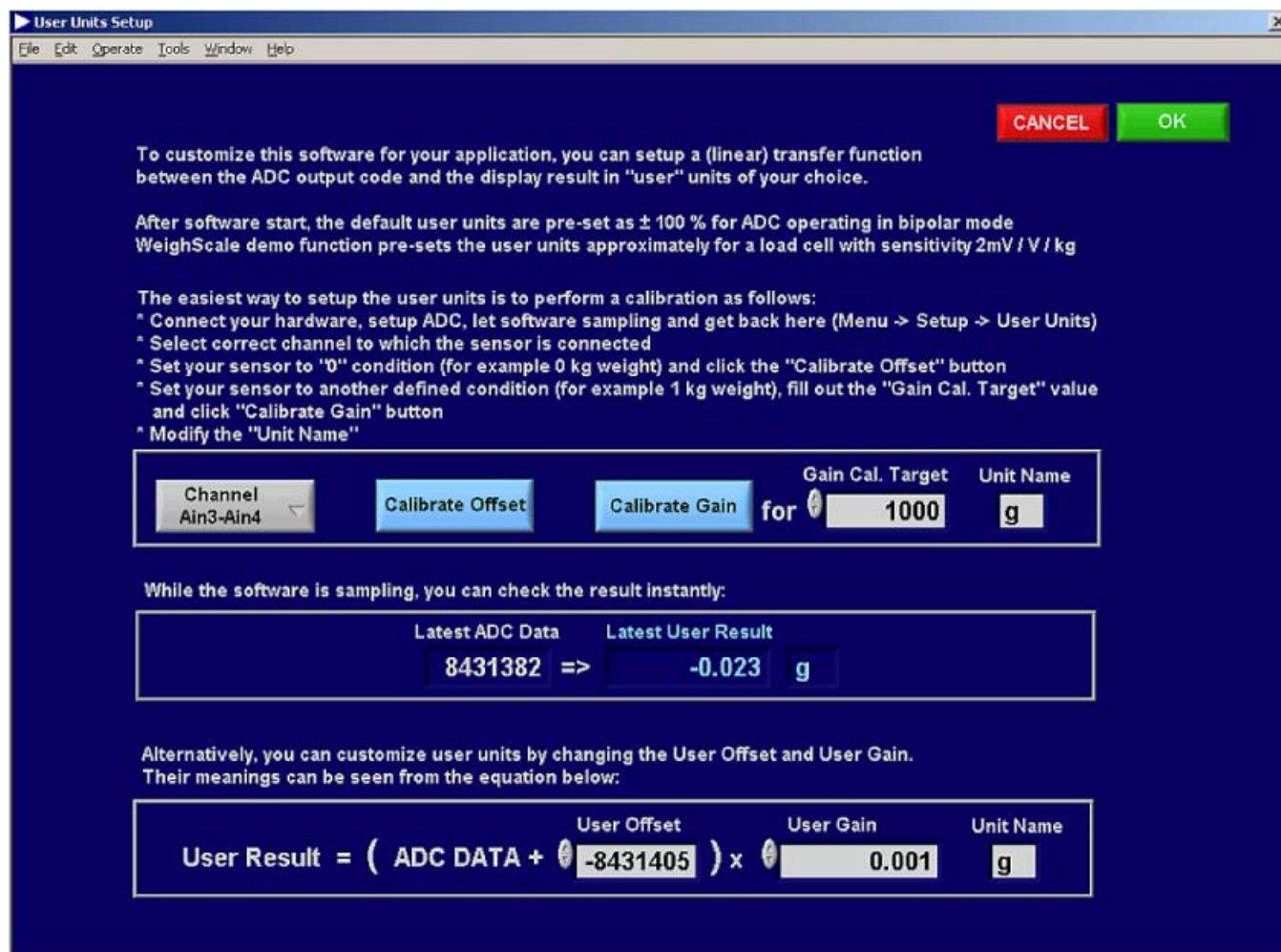
Figure 12. User Units Setup Window
