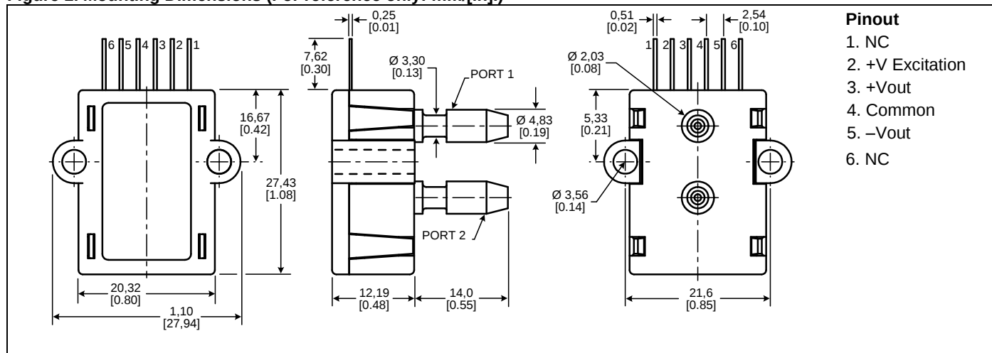
Figure 1. Mounting Dimensions (For reference only: mm/[in].)
