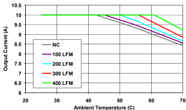
Figure 16. Derating Curves at Vo=2.5Vdc
