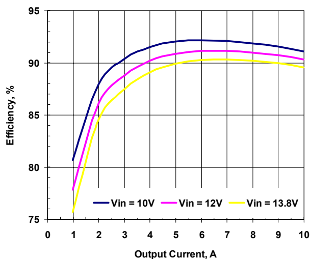
Figure 4. Efficiency vs. Load. Vout=3.3V
