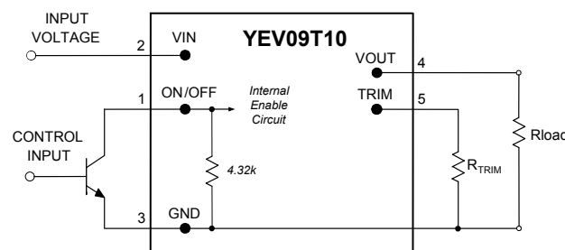
Figure 20. Circuit Configuration For ON/OFF Function
