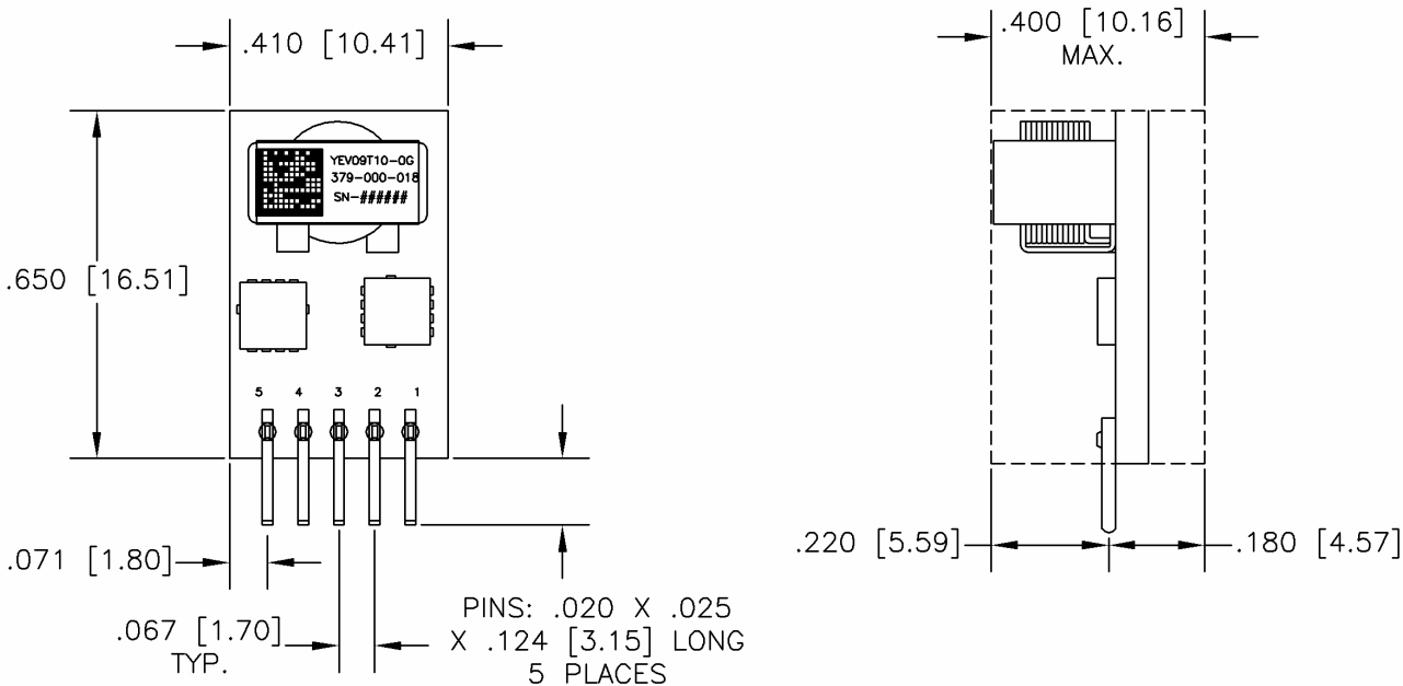
Figure 22. Mechanical Drawing
