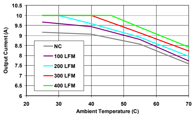
Figure 18. Derating Curves at Vo=5.0Vdc
