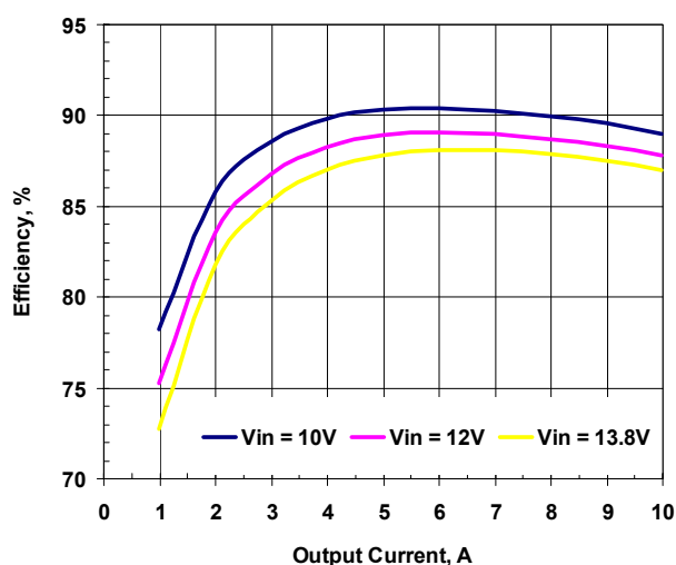
Figure 3. Efficiency vs. Load. Vout=2.5
