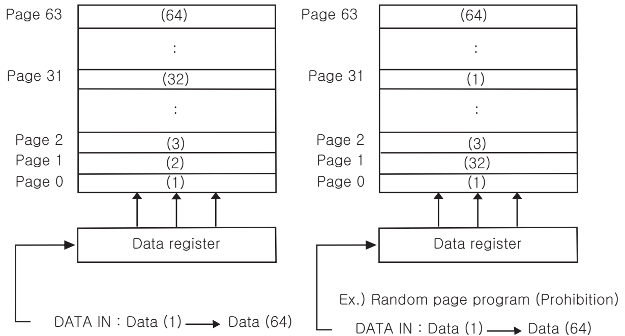
Figure 28: page programming within a block
