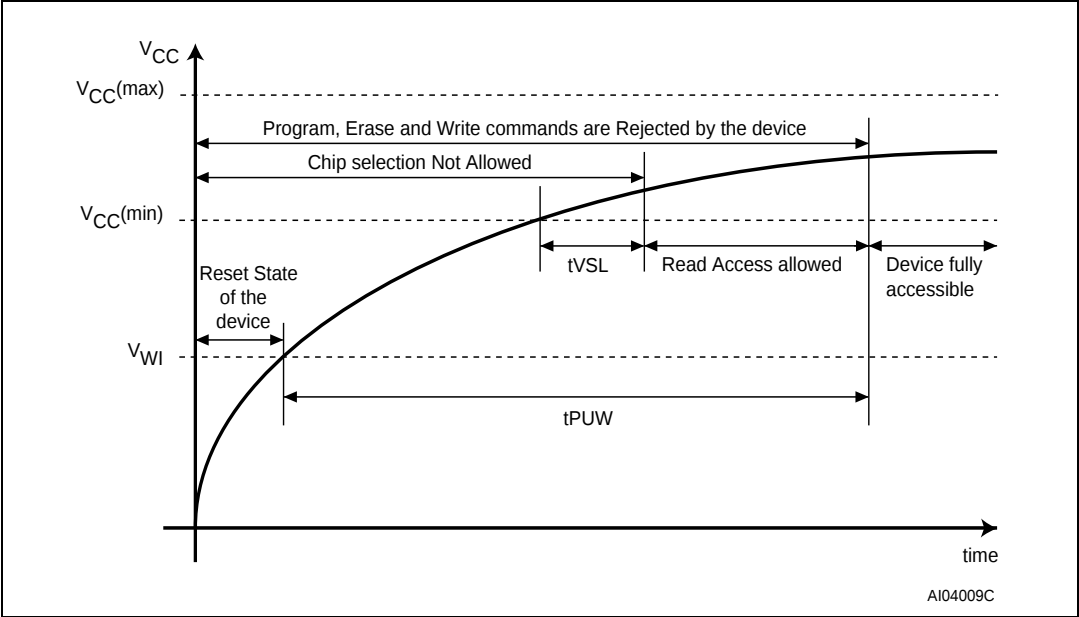
Figure 20. Power-up timing
