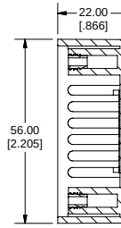
SECTION B-B
