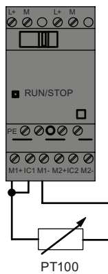
2-wire technique
