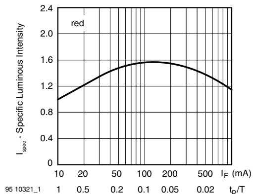
Figure 6. Spec. Luminous Intensity vs. Forw. Current/Duty Cycle
