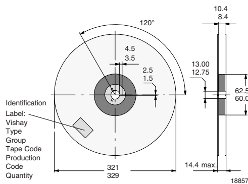
Figure 31. Reel Dimensions - GS18
