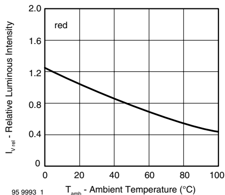
Figure 5. Relative Luminous Intensity vs. Ambient Temperature
