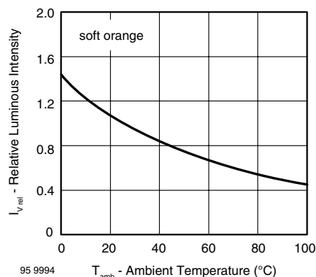
Figure 10. Relative Luminous Intensity vs. Ambient Temperature
